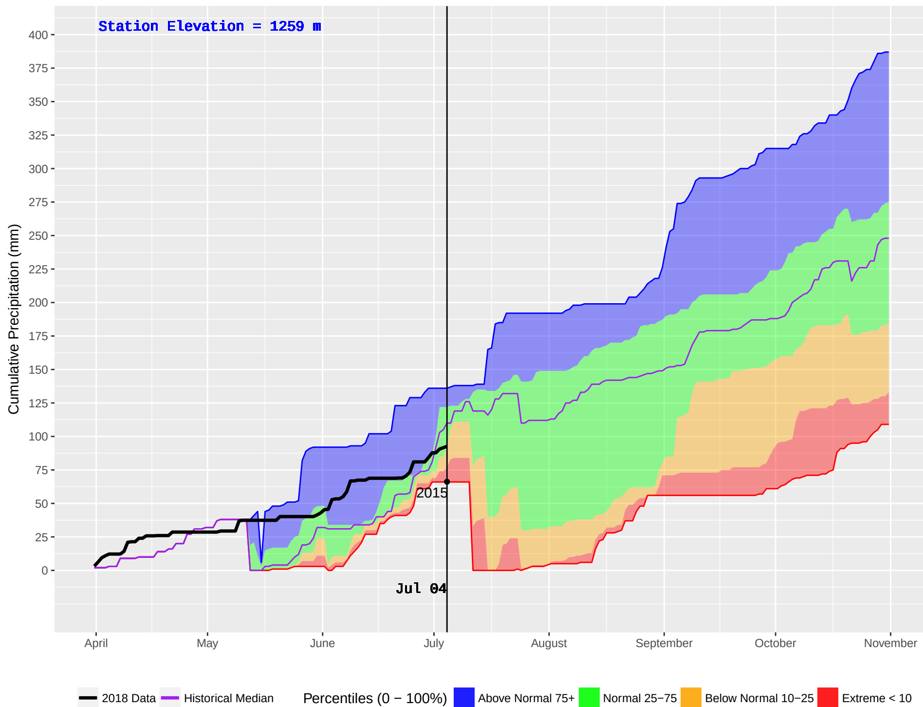
PARROTT (183) : Historical (1995–2016) and Current (2018) Noon Cumulative Precipitation
