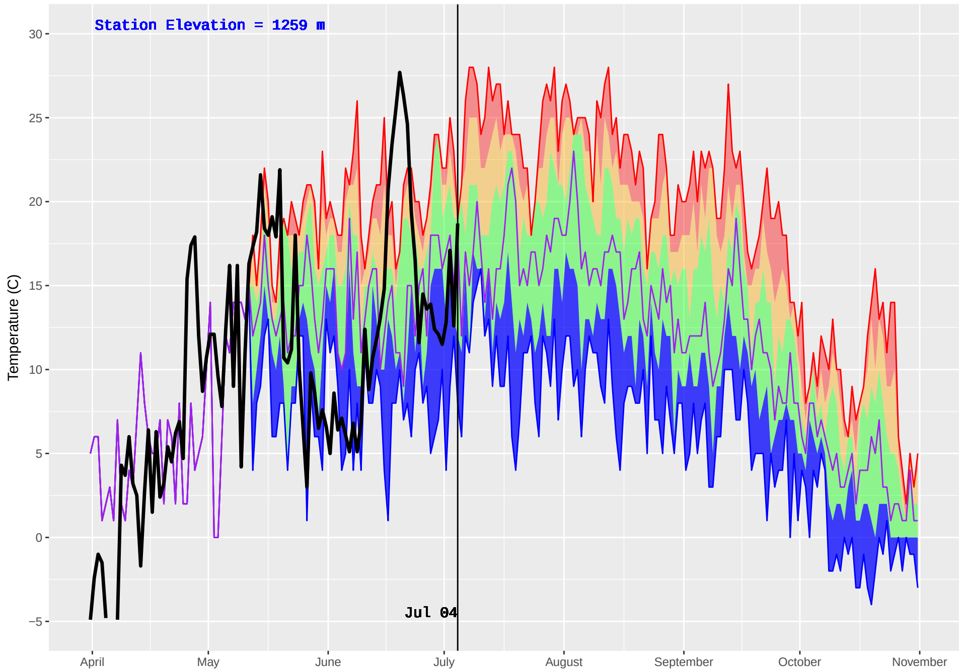
PARROTT (183) : Historical (1995–2016) and Current (2018) Noon Temperature
