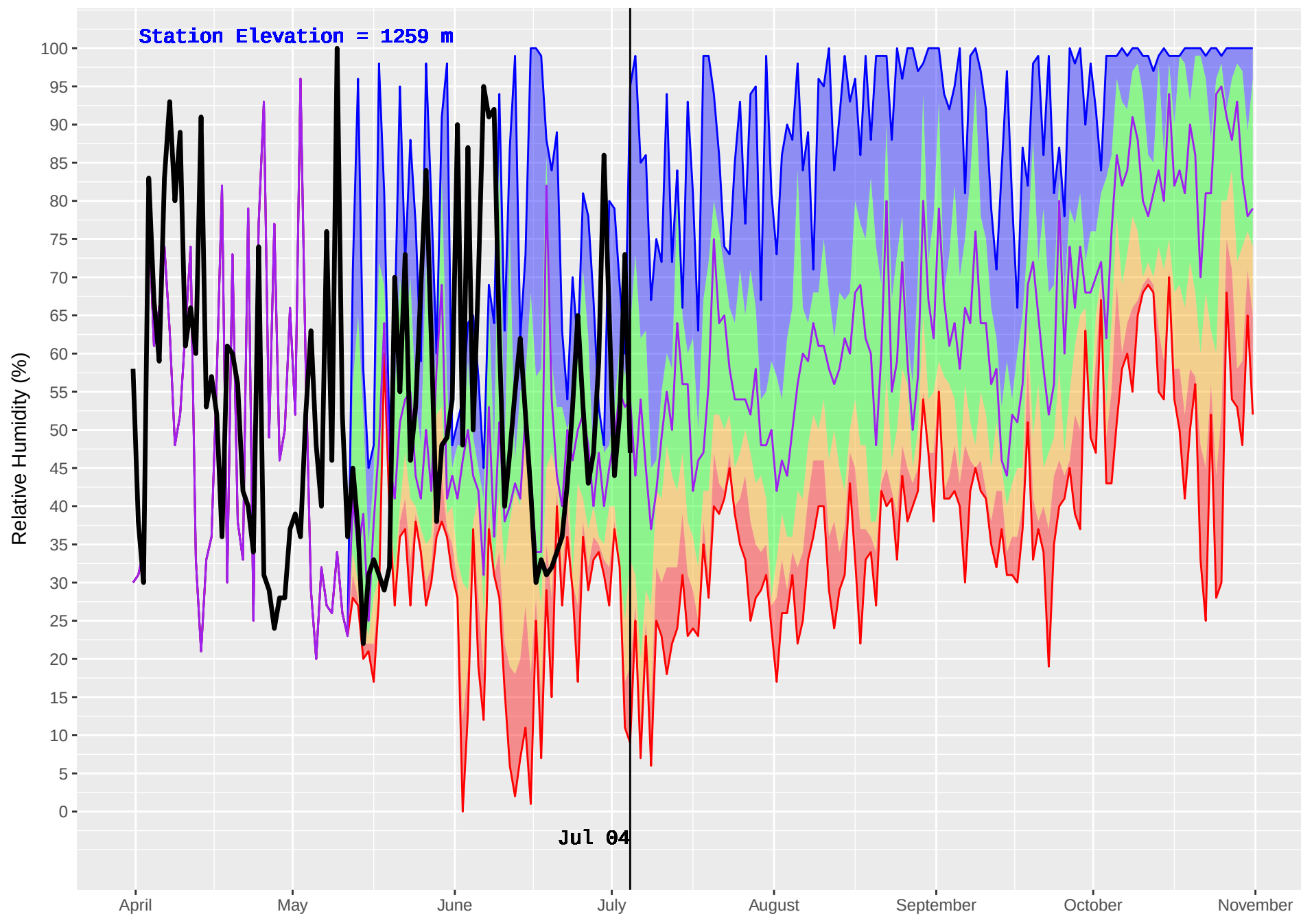
PARROTT (183) : Historical (1995–2016) and Current (2018) Noon Relative Humidity
